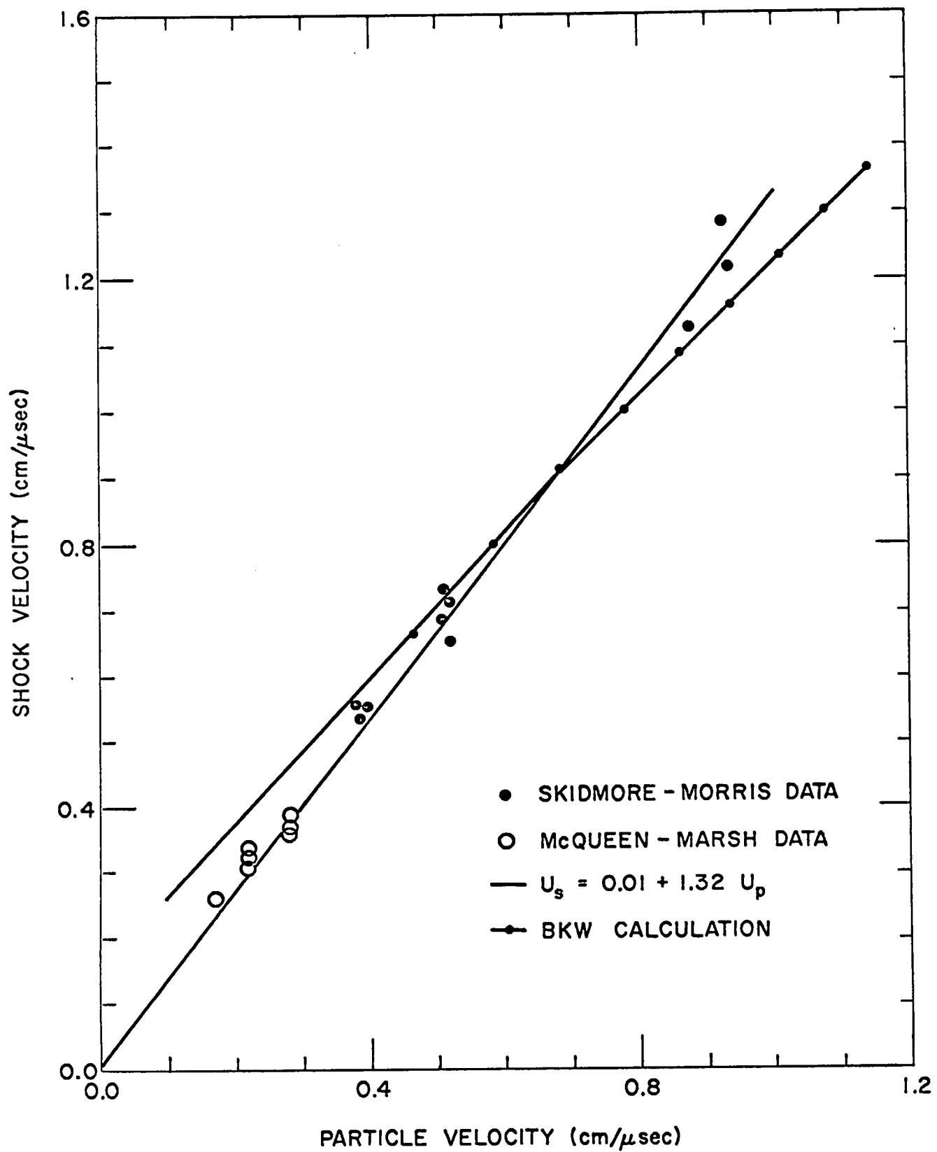
Fig. 1. The experimental and calculated Hugoniot curves for 0.32-g/cc polyurethane.
