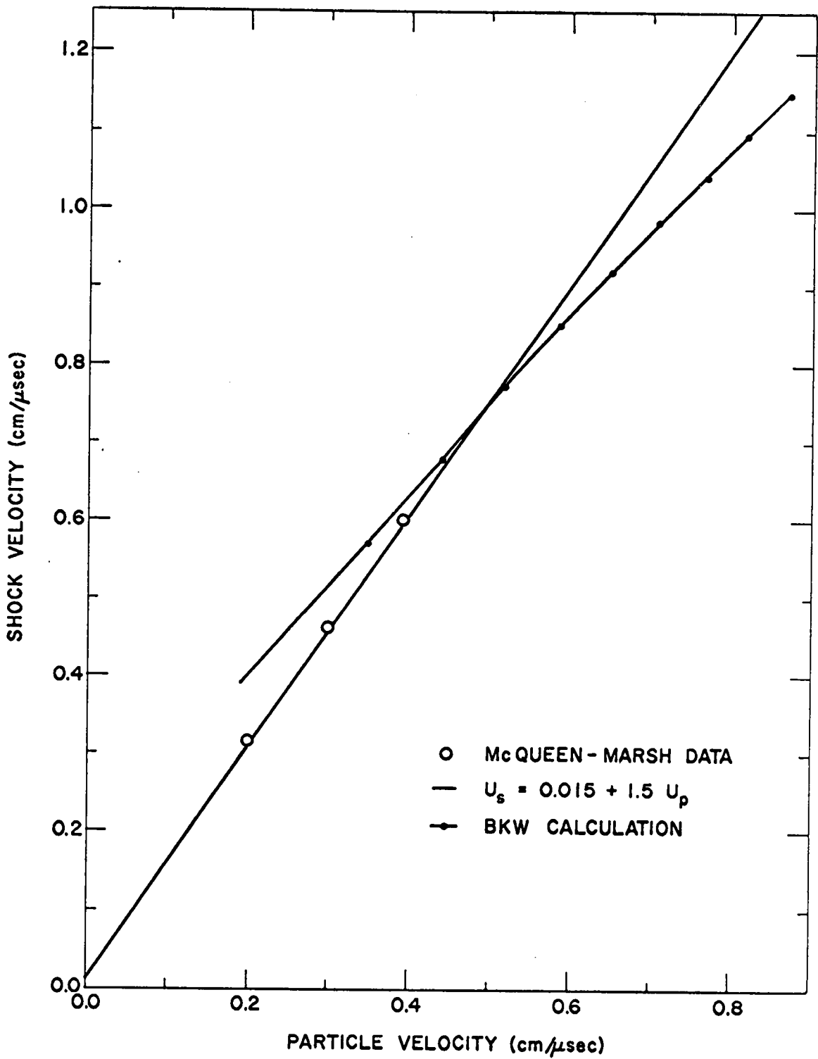
Fig. 2. The experimental and calculated Hugoniot curves for 0.5 g/cc polyurethane.
