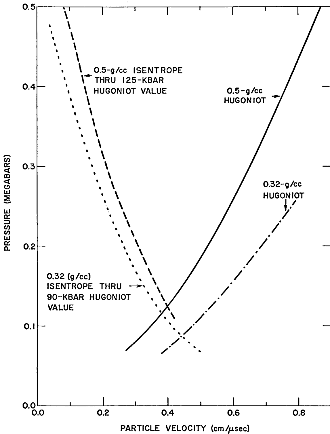
Fig. 3. The calculated BKW Hugoniot and isentropes for 0.5- and 0.32-g/cc polyurethane.
