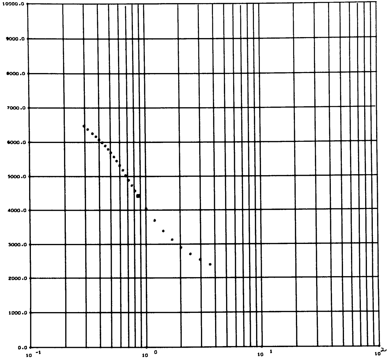
FOAMED MIXTURE OF URETHANE AND ADIPIC ACID TEMPERATURE - VOLUME ISENTROPE
